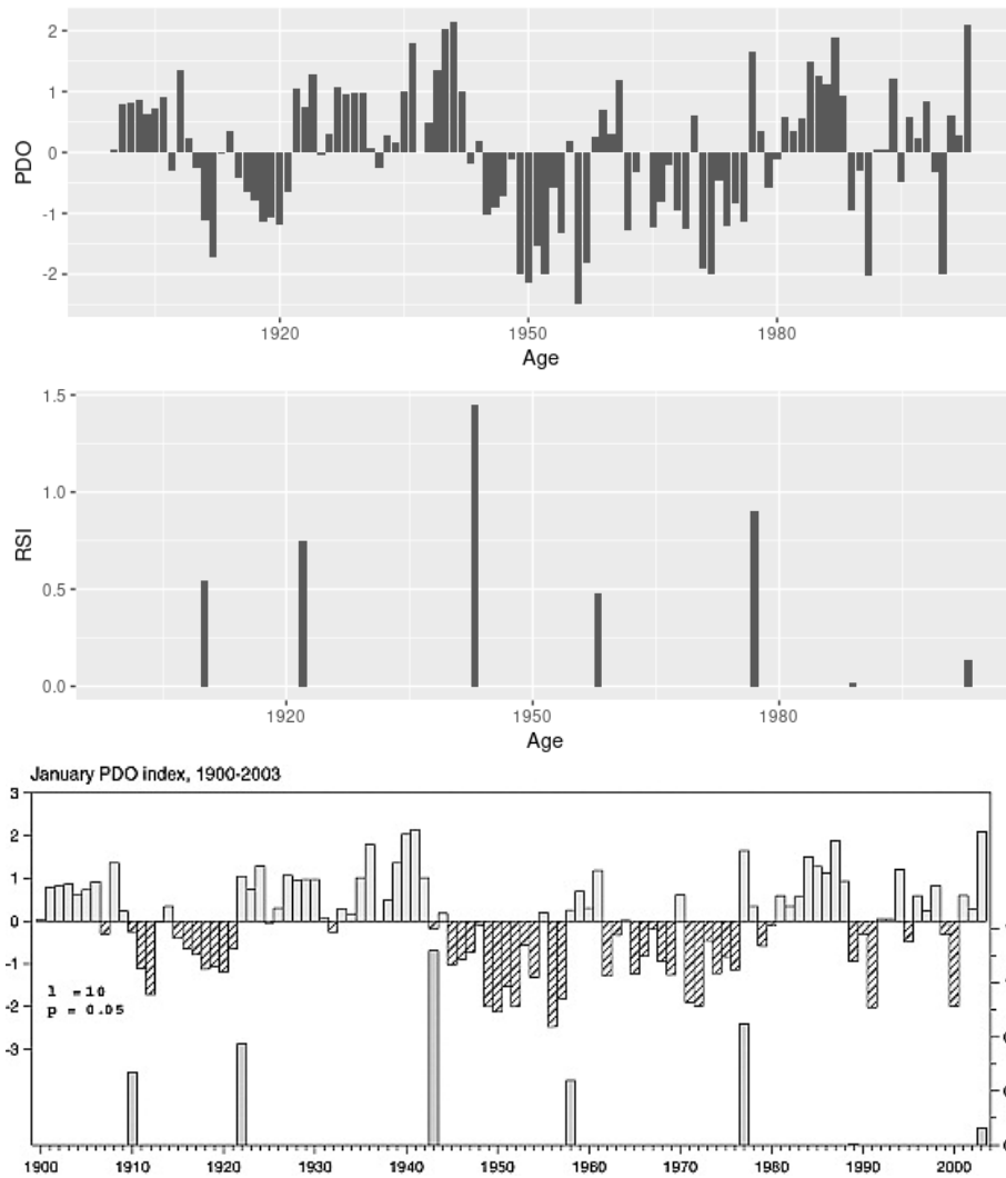
Figure 1: The RSI plot generated by rshift , and the plot of the same data from Rodionov [2004].
